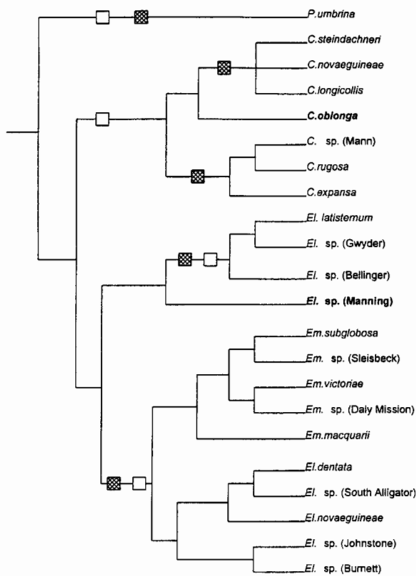
Figure 3. Occurrence of loss of exposed neurals mapped on the currently hypothesized phylogeny of Australian chelids (Georges and Adams, 1992). Open squares assume that in the Manning River Elseya neurals are ancestral and in C. oblonga they are secondarily derived. Hatched squares assume that both C. oblonga and Elseya sp. (Manning) retain ancestral neurals. Note: Elusor macrurus and Rheodytes leukops have been left out of this phylogeny for two reasons, 1) they were inadequately resolved (forming a trichotomy with the Elseya dentata – Emydura groups) and 2) they will have no effect on the neural character state, both species lacking exposed neurals.
