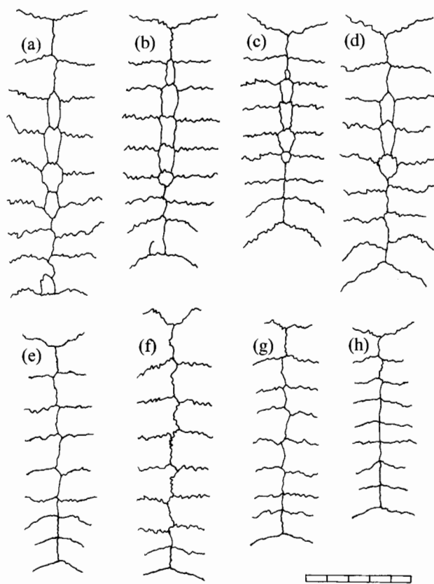
Figure 1. Comparison of the neural region of the dorsal carapace of the sibling species pair Elseya sp. aff. latisternum (Manning) (upper row, a to d) and Elseya sp. aff. latisternum (Bellinger) (lower row, e to h). Scale = 5 cm. (a) AM 123042, (b) QM 59290, (c) QM 59289, (d) AM 123040, (e) AM 138387, (f) AM 138388, (g) UM 02016, (h) UM 02017.
