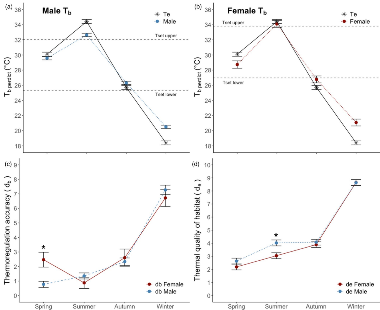
FIGURE 2 Mean seasonal environmental temperature ( T_e ), thermal preference ( T_{set} ) and predicted body temperature ( T_{b, Predict} ) for male (a) and female (b) Pogona vitticeps . Accuracy of thermoregulation ( d_b ) between sex (c), where low d_b denotes body temperature closer to thermal preference. The thermal quality of habitat ( d_e ), measured using copper models that account for sex differences in thermal preference (d). Low d_e values indicate more environmental temperatures fell within T_{set} (i.e. favourable thermal environment). Error bars for all panels are \pm 1 standard error of the mean. The asterisk symbol indicates a significant difference ( p < 0.01 ) when comparing mean differences between sexes for that season.
